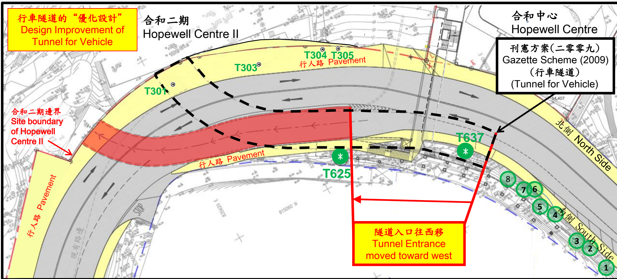
優化設計 (地面) Design Improvement (Ground Level)
