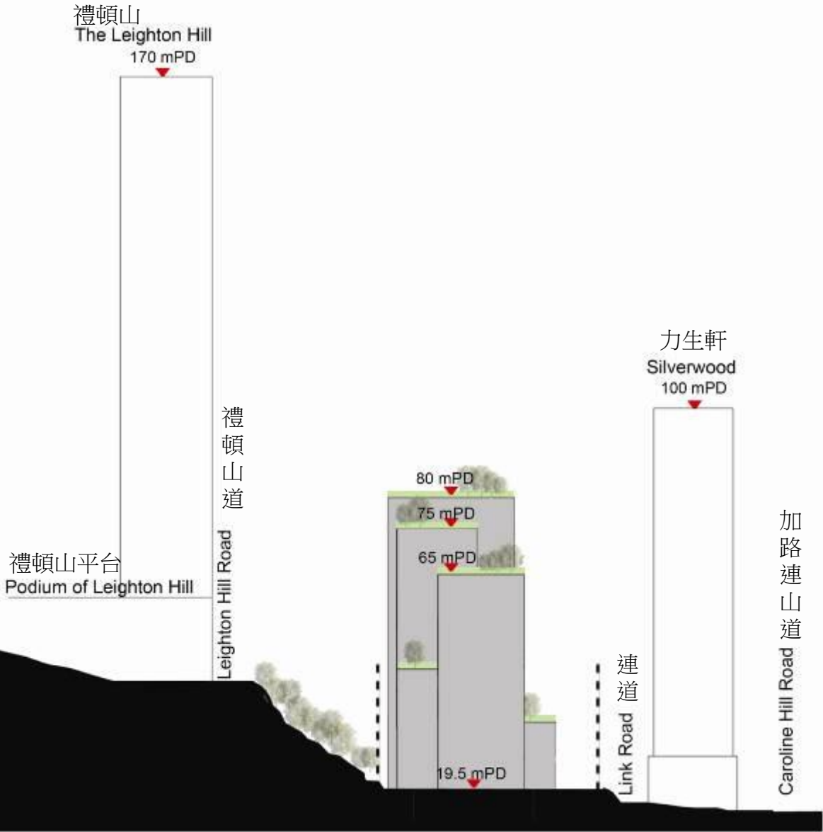
Section c-c'
